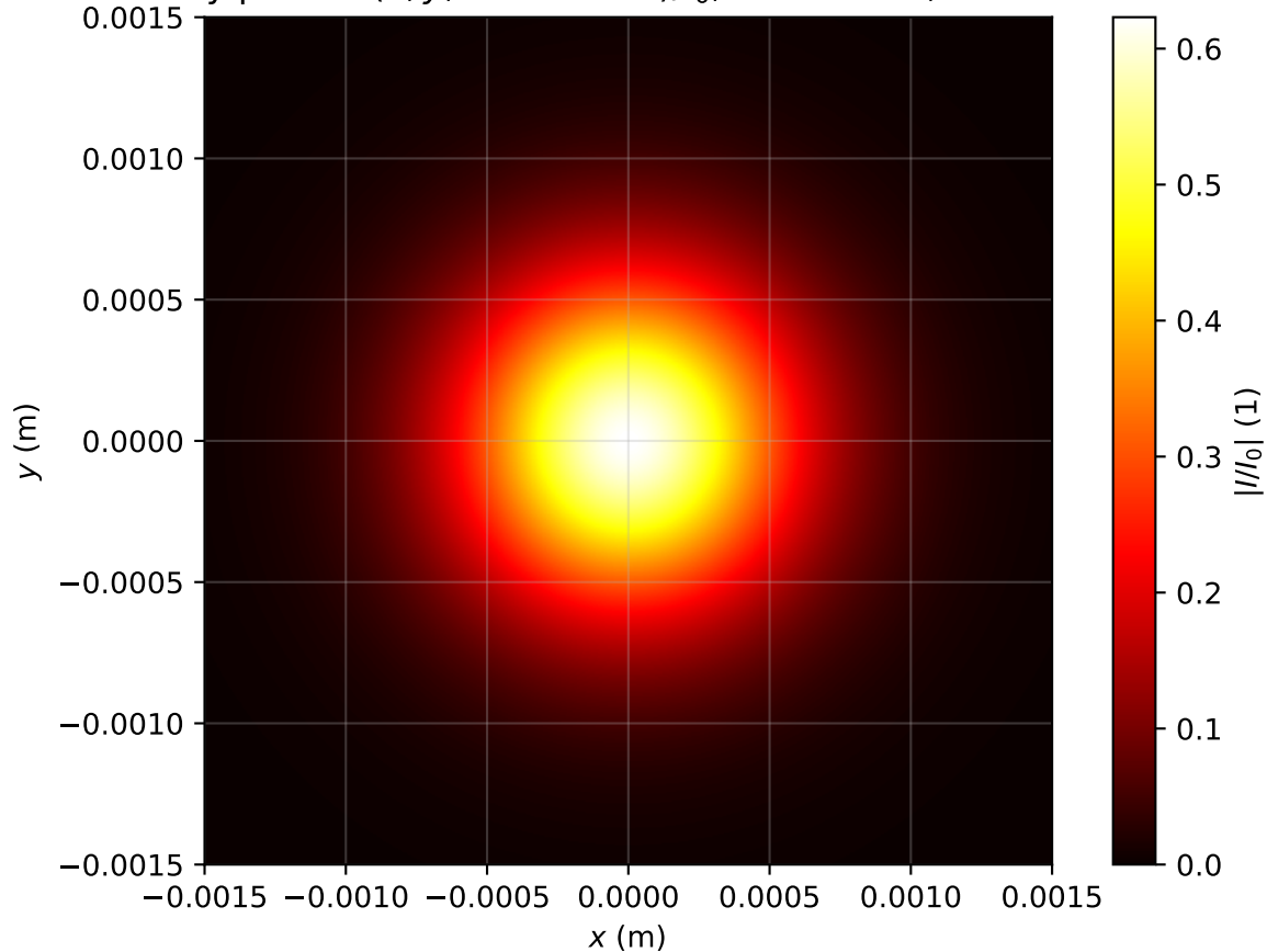
Intensity profile I(x, y, z = 2.388m)/I_0 , P_{in}=0.4P_{cr} , artificial time
